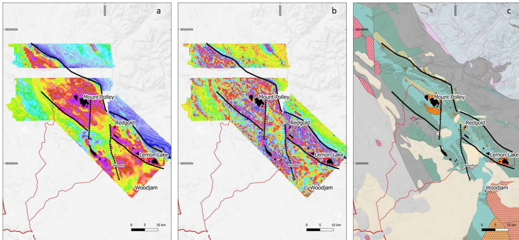
Regional Airborne Magnetic Interpretation. Total field (a), and vertical gradient magnetics (b), regional geology (c)(refer to figure 3 for colour scheme); black lines - interpreted magnetic domains, dotted lines - faults. Note that late Triassic plutons at Mount Polley, Redgold and Lemon Lake correspond with very high magnetic intensity anomalies (solid black). Magnetic interpretation suggests Mount Polley, Redgold and Lemon Lake are on a common NW-SE geological trend. Magnetic Source Data: BCGS Open File 2004-09, Horsefly Multisensory Geophysical Survey Parts of NTS 93A/3,5,6,11 Shives, R.B.K. et. al. Geological Survey of Canada, Cathro, M., B.C. Ministry of Energy and Mines
