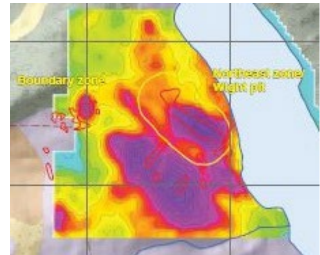
Coincident chargeability and mineralization at Mt Polley
