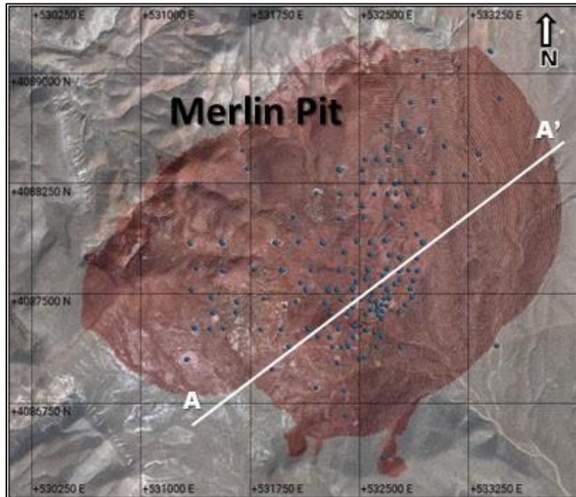
Figure 2: Plan view map of the 2024 Merlin Pit Design based on a gold price of US$1,900/oz Mineral resource. 3 Drill hole collars in blue.
