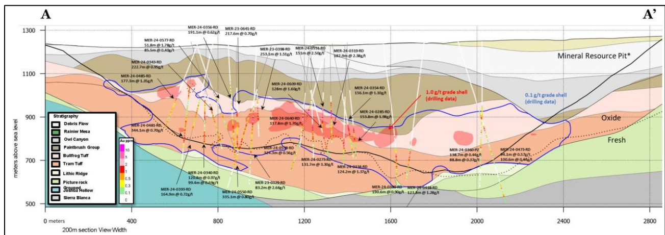
Figure 3: Long section looking NW across the Merlin Deposit 3 (Section location shown on Figure 2)
